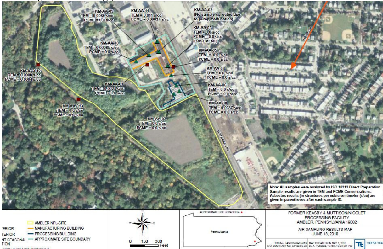
Figure 13 – Ambient air sampling locations for the former K&M Buildings (while no ABS occurring in the buildings)
