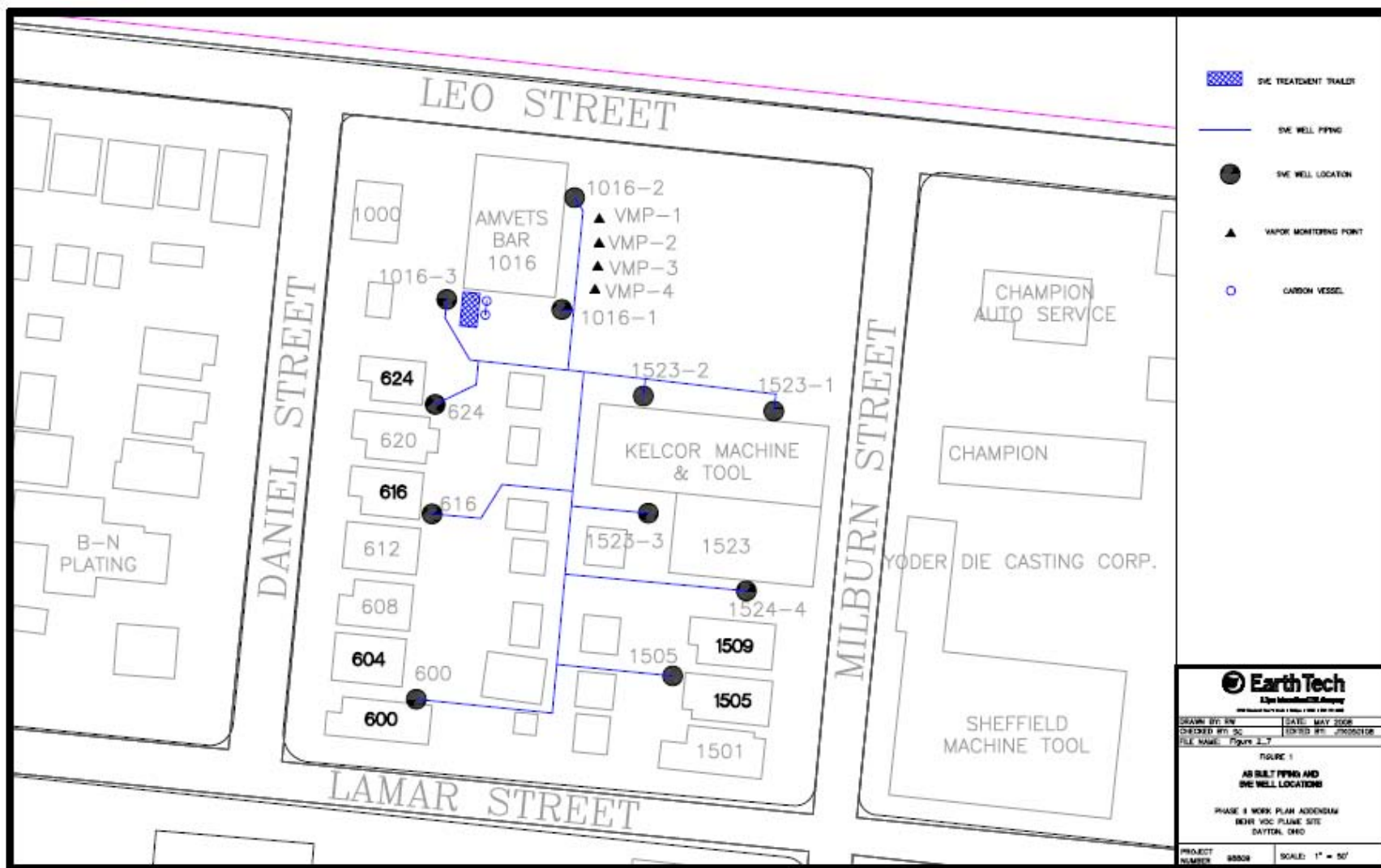
Figure 6 As Built Soil Vapor Extraction
