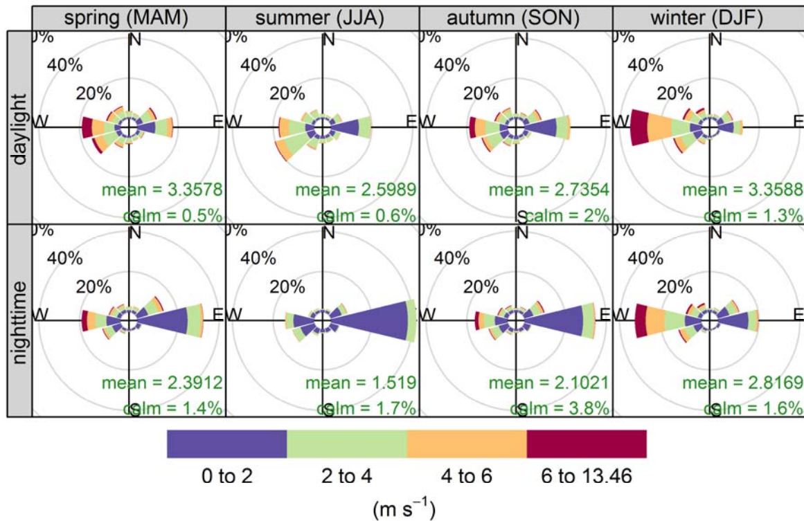
Figure 3: AERMET Surface File Diurnal/Seasonal Wind Roses
