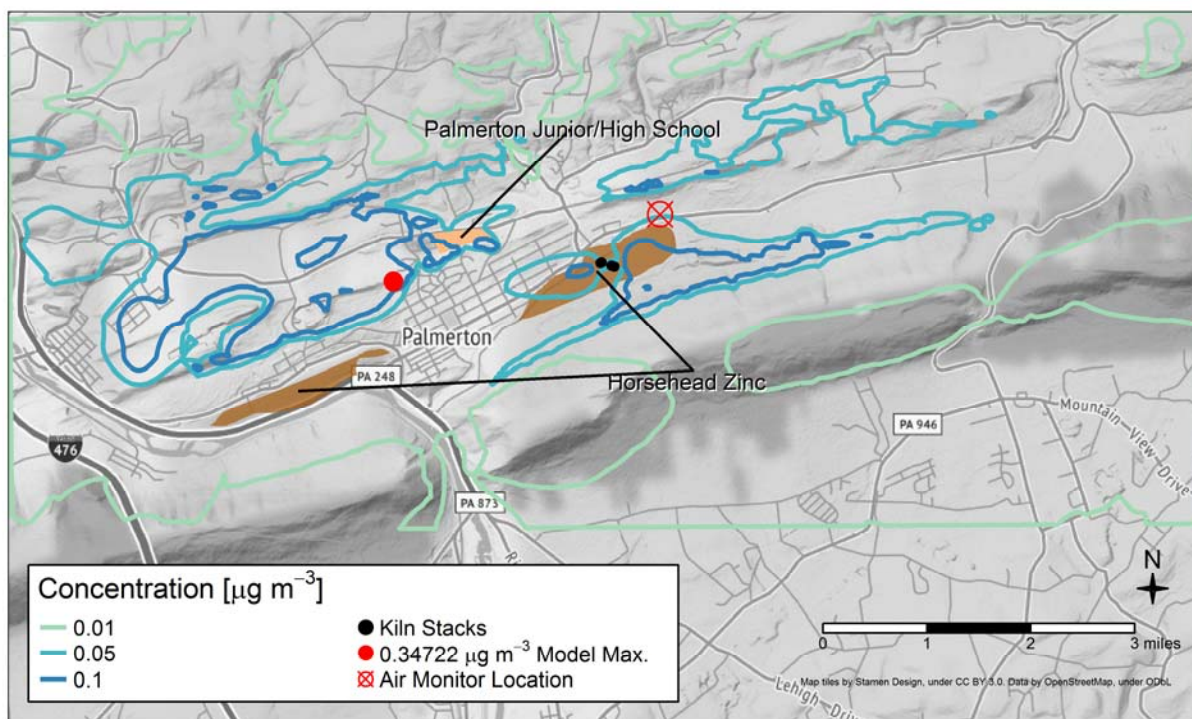
Figure 10: AERMOD 95% 24-Hour Average Lead Concentration
