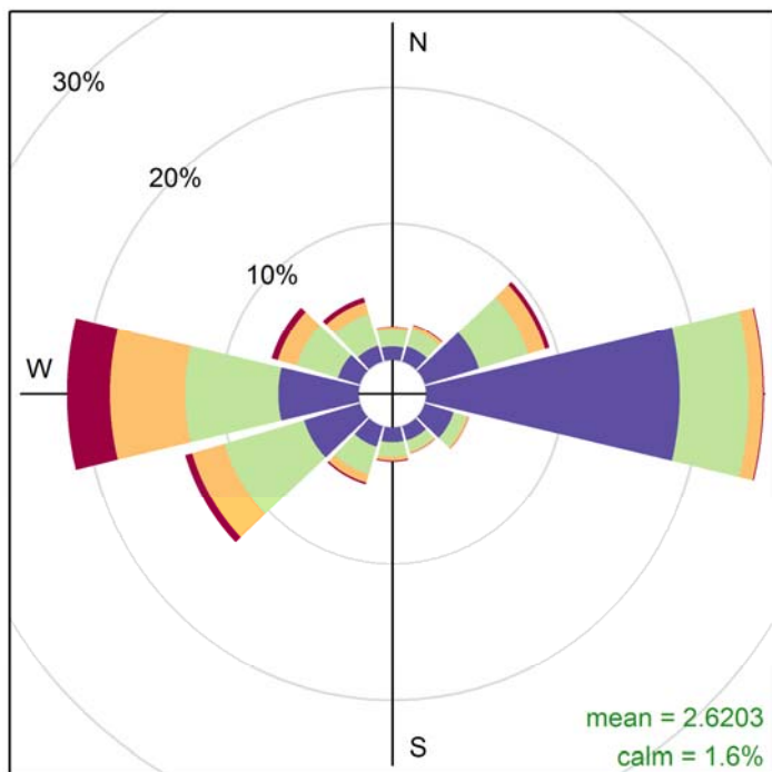
Figure 2: AERMET Surface File Wind Rose
