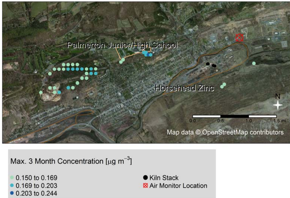
Figure 8: AERMOD Receptors Exceeding NAAQS
