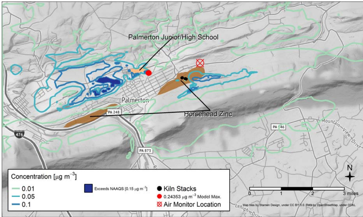
Figure 7: AERMOD Highest Rolling 3-Month Average Lead Concentration
