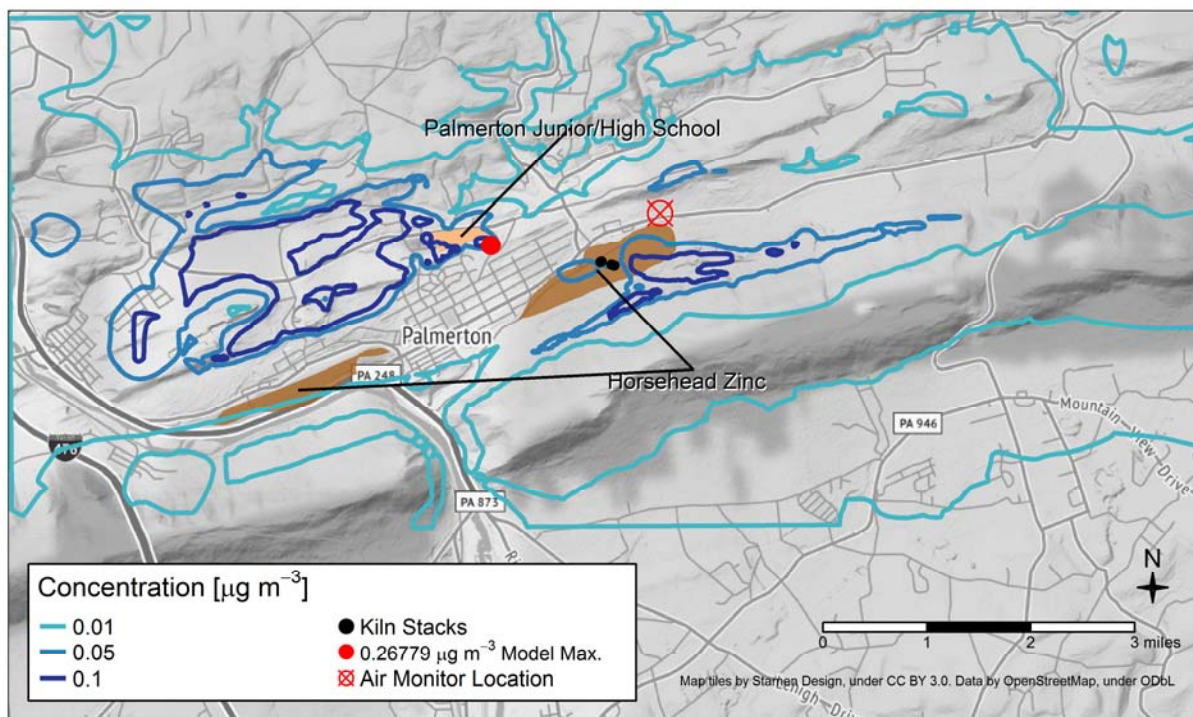
Figure 6: AERMOD Highest Monthly Average Lead Concentration
