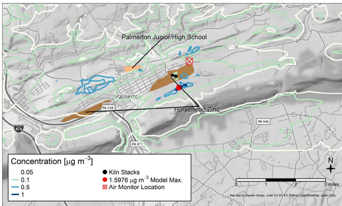
Figure 9: AERMOD Highest 24-Hour Average Lead Concentration
