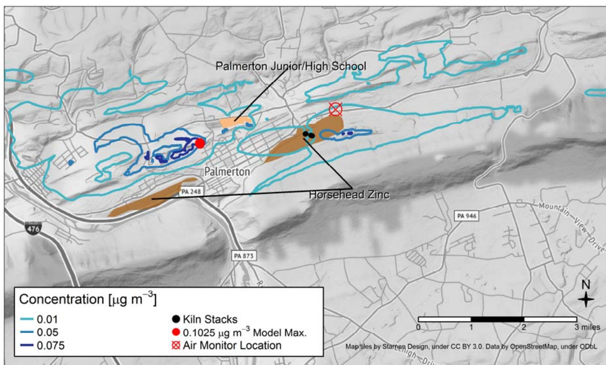
Figure 5: AERMOD Predicted Annual Lead Concentration
