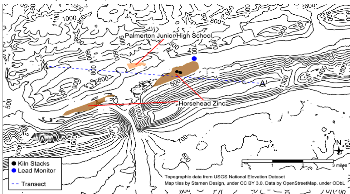
Figure 1: Palmerton, PA Terrain Map
