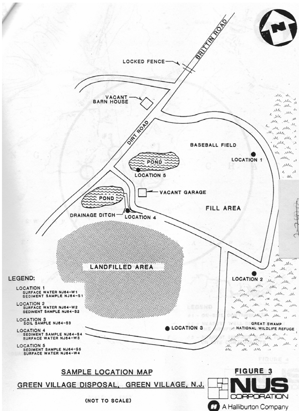
Figure 4: Aqueous and soil/sediment sample location map (NUS 1985)
