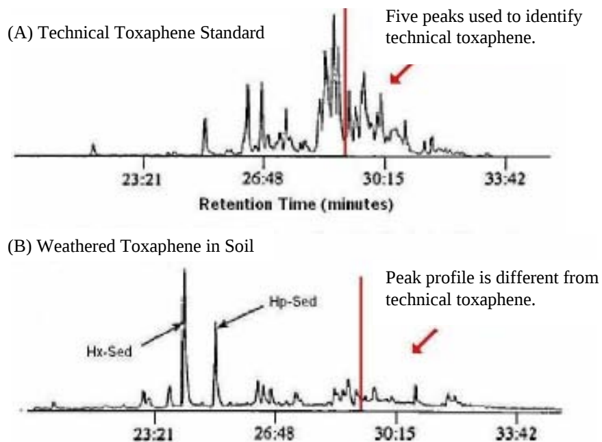
Figure 1: Chromatograms for technical (A) and weathered (B) toxaphene using EPA Method 8081 (EPA 2005).
