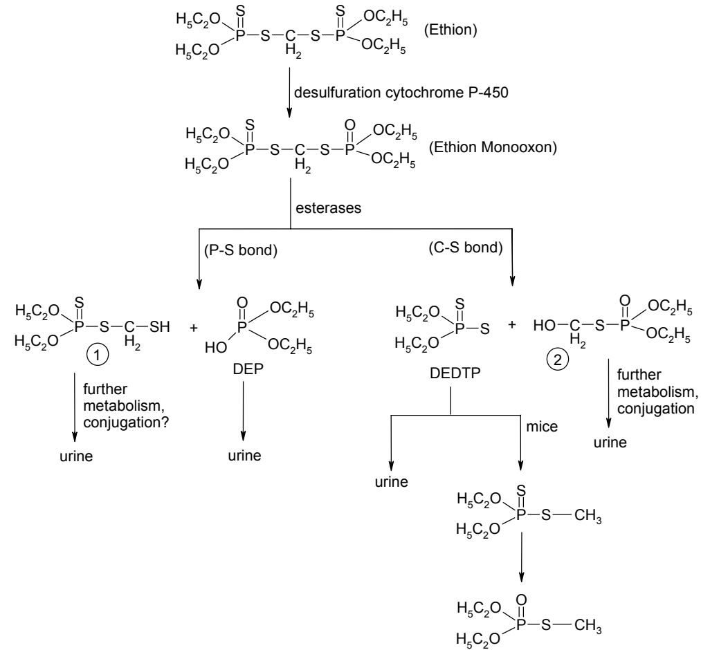
Figure 2-2. Proposed Mammalian Pathways of Ethion Biotransformation
