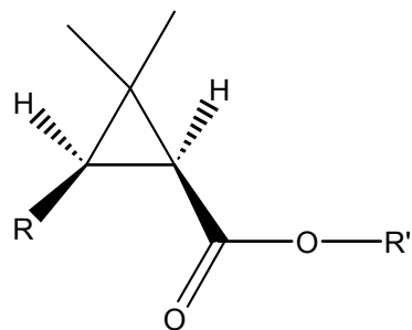
1S cis configuration
