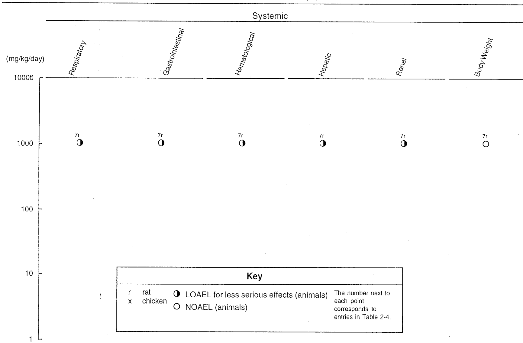
Figure 2-4. Levels of Significant Exposure to Mineral Oil Hydraulic Fluids - Oral (cont.) Intermediate (15-364 days)
